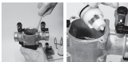
E- Remove the downstream valve (7).
